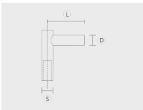
Mounting arm - 1 side PTCS
